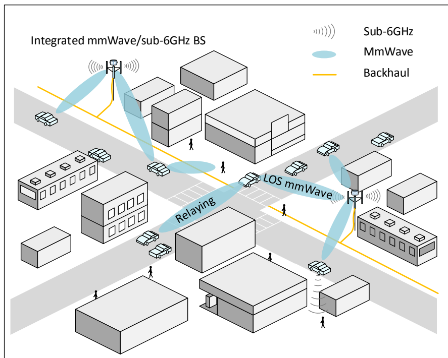
Figure 1. Relaying in the integrated mmWave/sub-6GHz 5G network.
