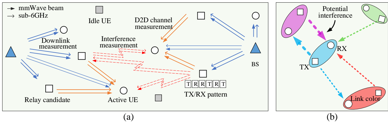
Figure 3. (a) A discovery/measurement framework for the integrated mmWave/sub-6GHz networks with D2D relaying; (b) Local interference graph constructed by interference measurement. Each Relay-to-UE link uses a specific fraction of the D2D resources, indicated by a color. Here the blue and the purple D2D pairs are close neighbor links, so they should not use the same color to avoid strong interference.
