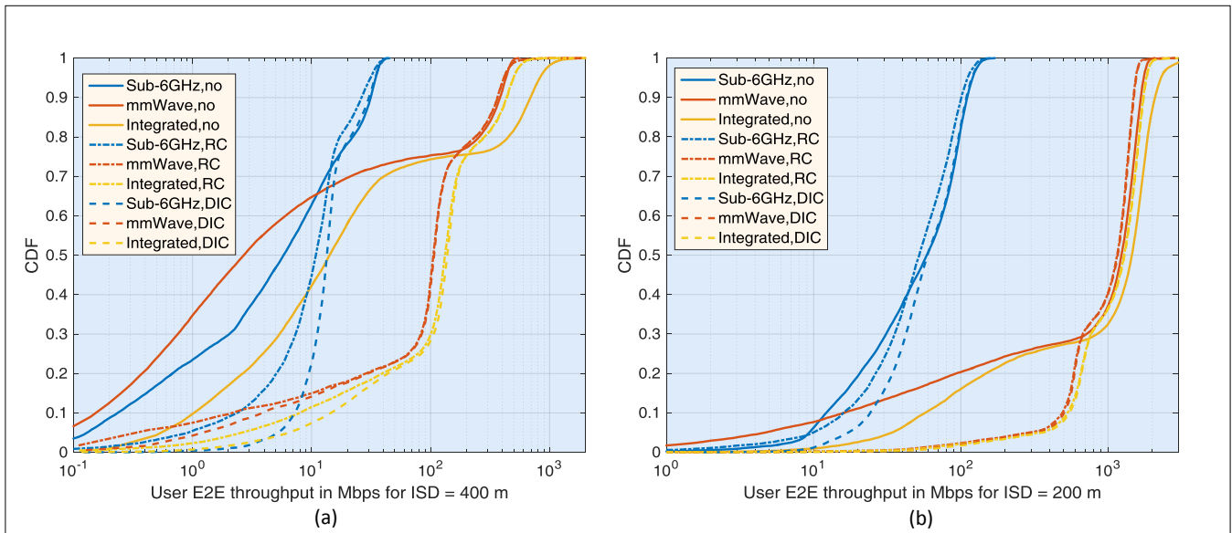
Figure 5. (a) CDF of user E2E throughput in standalone sub-6GHz, standalone mmWave and the proposed integrated mmWave/sub-6GHz (Integrated) deployments with ISD=400 m, for no relaying, relaying with random coloring (RC-relaying), and relaying with distributed interference coordination (DIC-relaying); (b) CDF of user throughput in sub-6GHz, mmWave and integrated deployments with ISD=200 m, for no relaying, RC-relaying and DIC-relaying.
