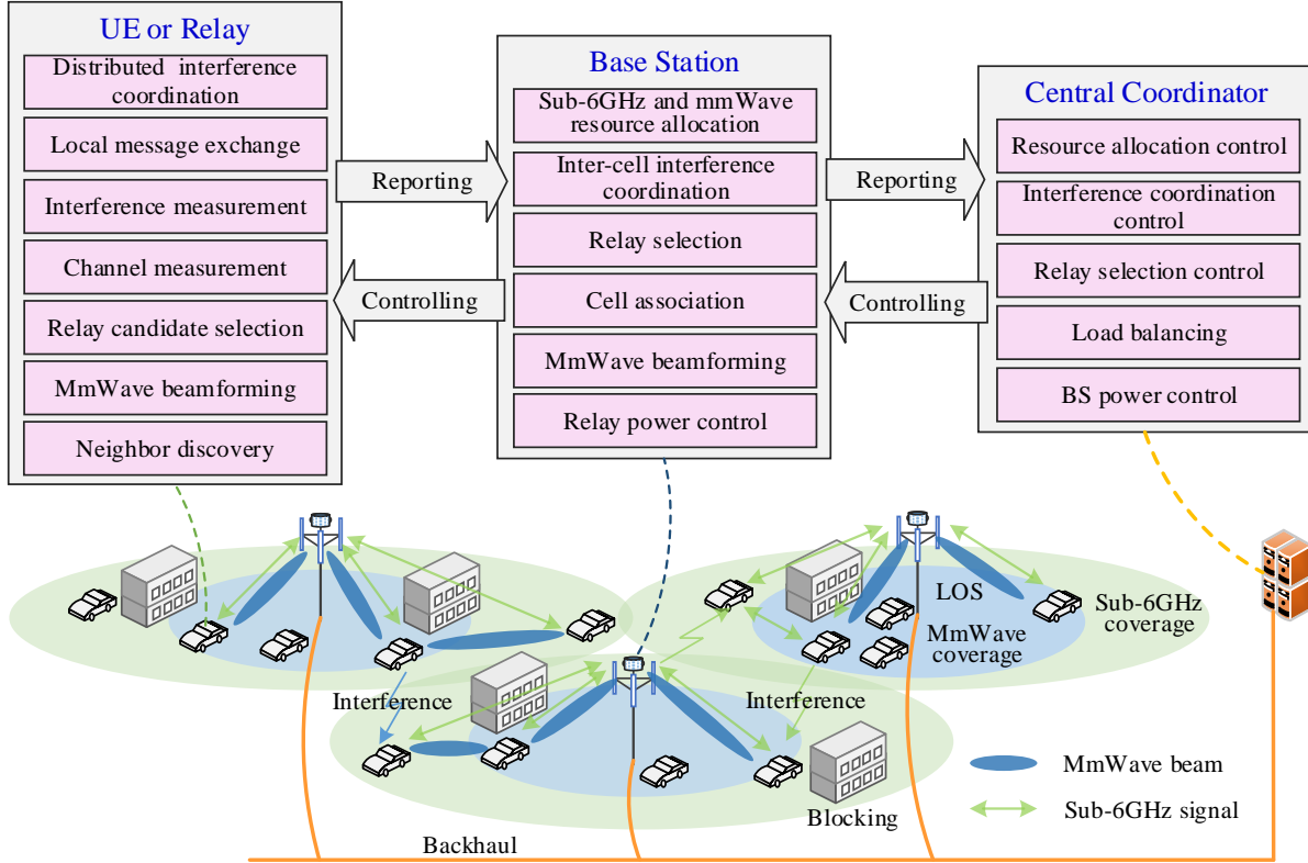
Figure 2. A hierarchical control framework for relaying-enabled integrated mmWave/sub-6GHz networks.
