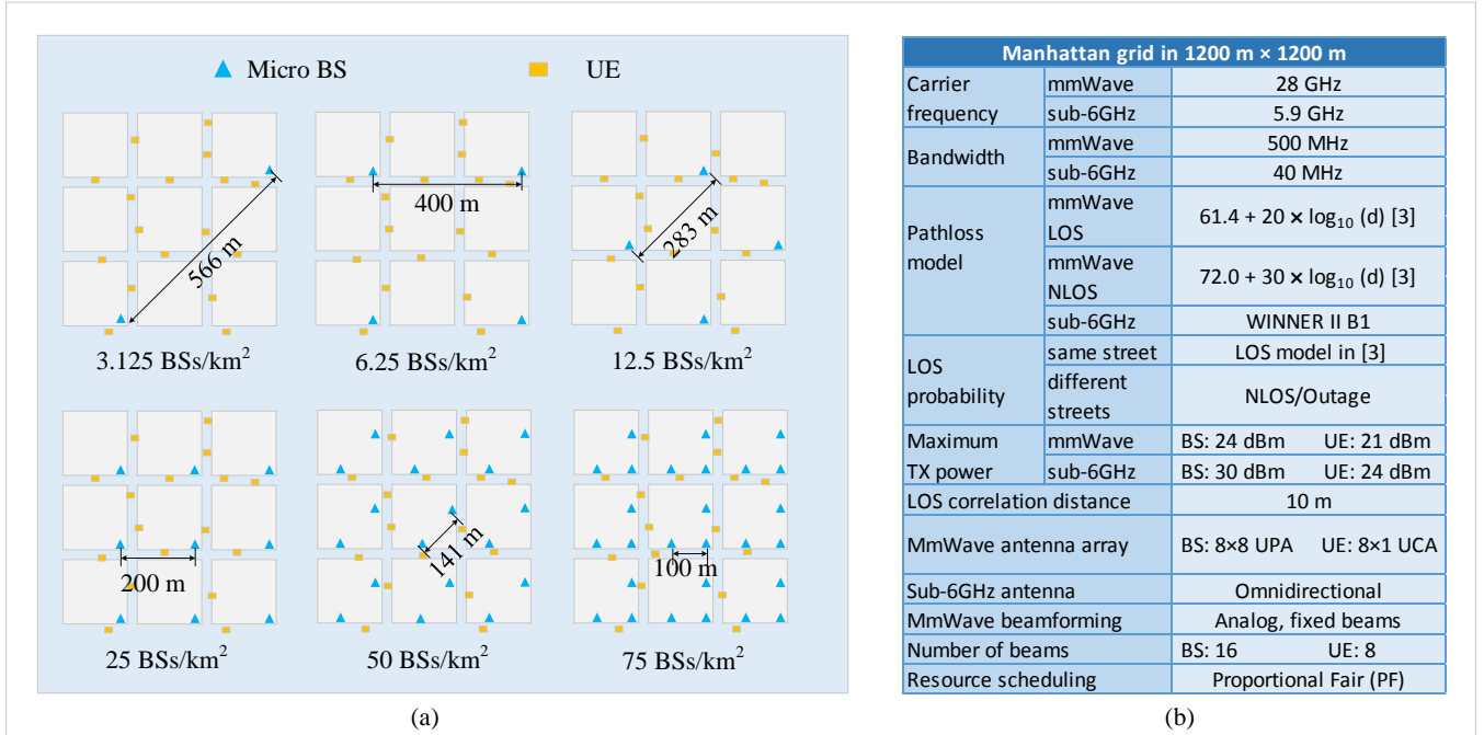
Figure 4. (a) Six BS deployment scenarios with different ISDs and correspondingly different BS densities in Manhattan grid; (b) Simulation parameters.
