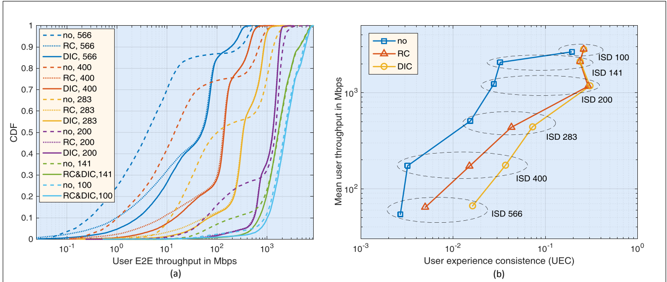
Figure 6. (a) CDF of user E2E throughput in the integrated mmWave/sub-6GHz deployment for six ISD alternatives; (b) 2D plot of UEC vs mean throughput in the integrated mmWave/Sub-6GHz deployment for six ISD alternatives, using a log-log scale.
