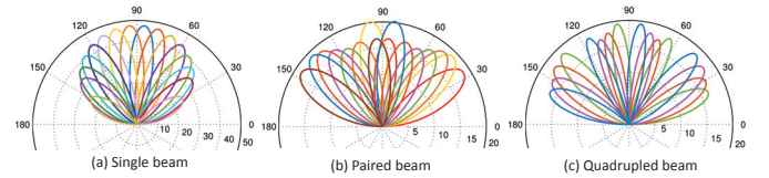
Fig. 3. Beam pattern for |\mathcal{B}_i| = 16, 8, 4
